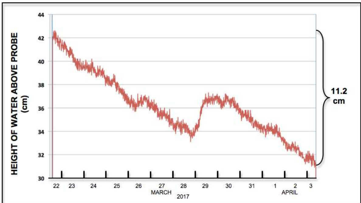
Figure 15. Water level on pond March 22 to April 3, 2017.
