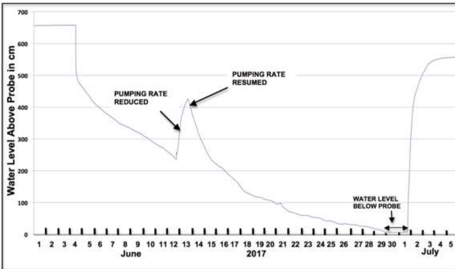
Figure 21. Water level in well during 27.3-day pumping test.
