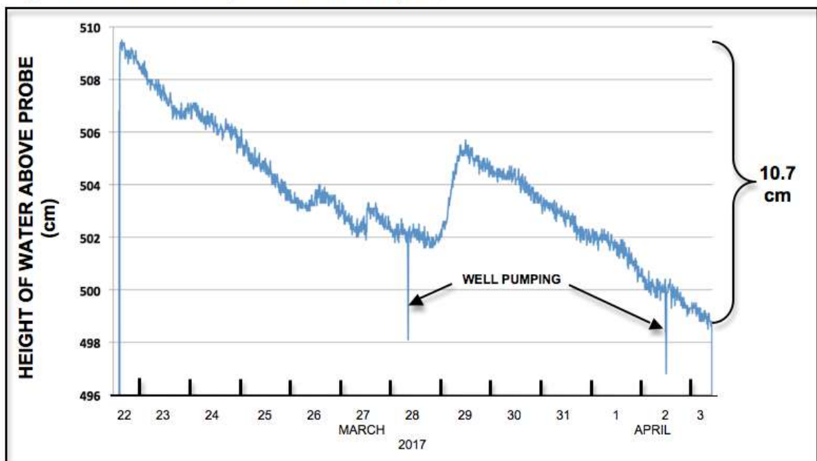
Figure 16. Water level in well March 22 to April 3, 2017.
