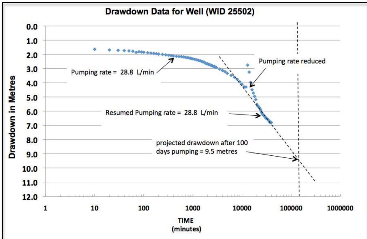
Figure 20. Drawdown data results for 27.3-day pumping test on well, June 4 to July 1, 2017.
